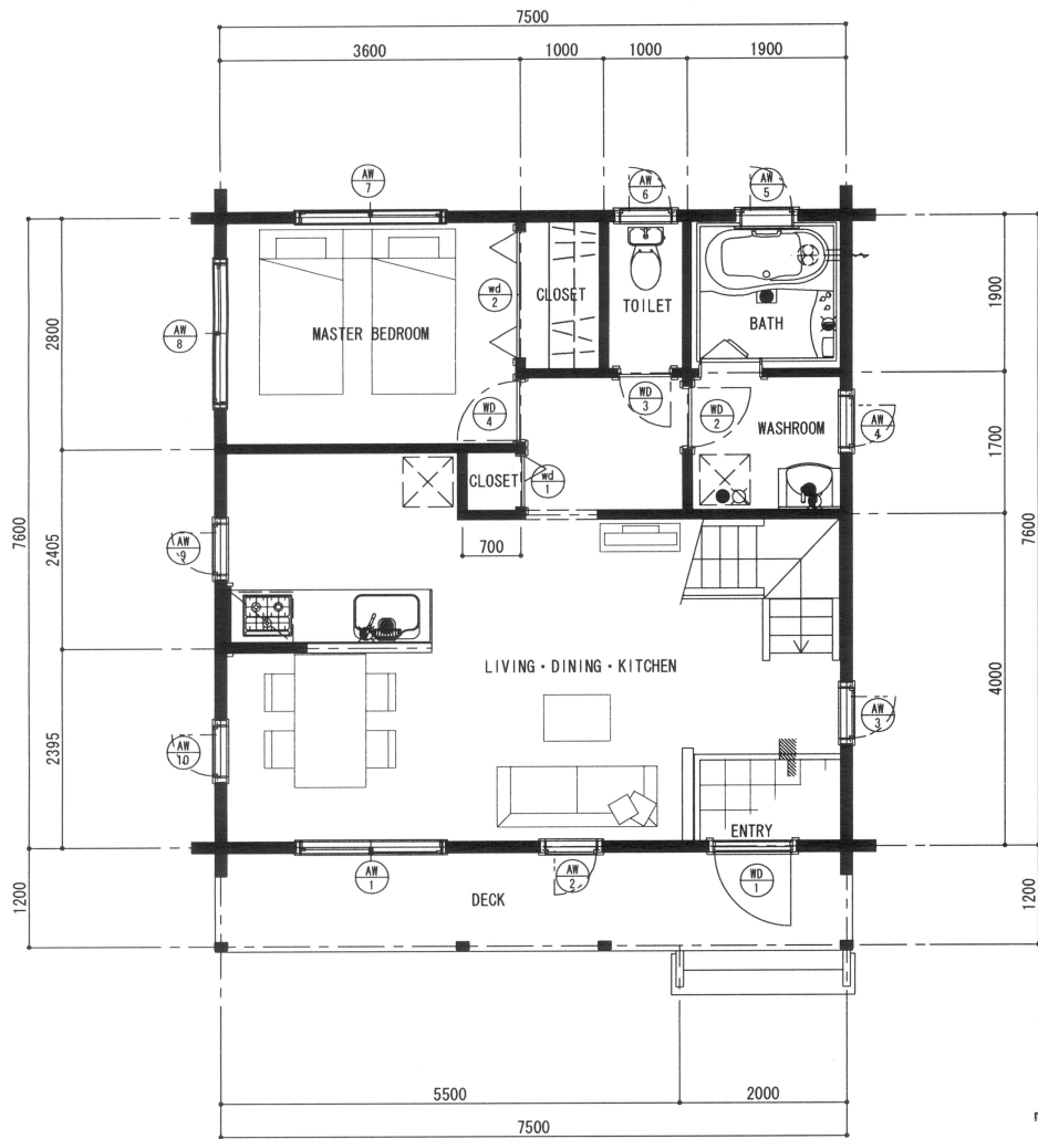
MAIN FLOOR
