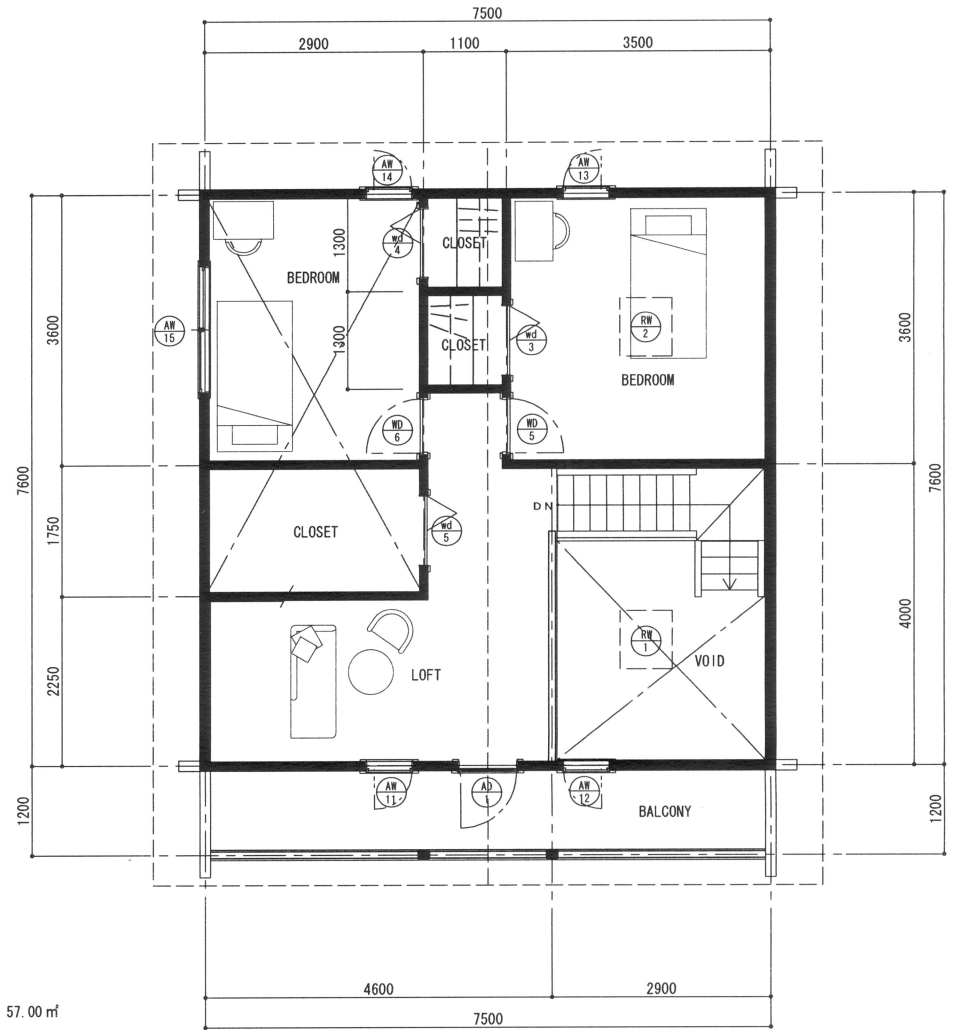
UPPER FLOOR
